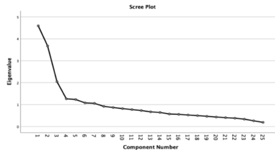
Figure 1: Scree plot for factors extracted
