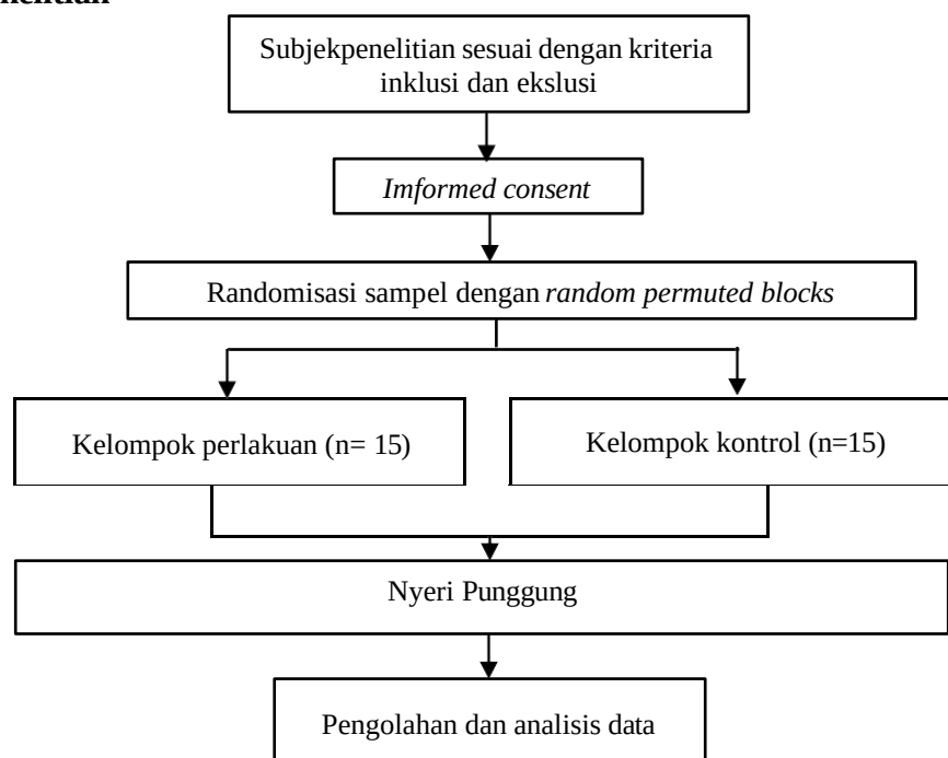
Gambar 4.2. Alur penelitian
