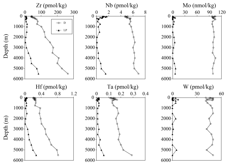
Fig. 3. Vertical profiles of D and LP-metals at station K1.
